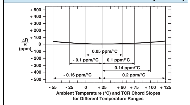
FIGURE 1 - TYPICAL RESISTANCE/TEMPERATURE CURVE (Z-FOIL)
